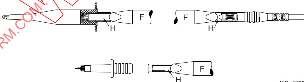
Figure 3c – Partially mated PROBE ASSEMBLY (see 6.2 and 6.4.1 b))
