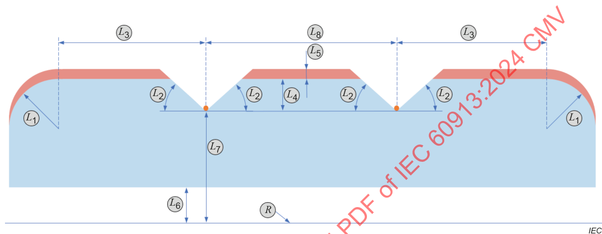
Figure E.4 – Clearance gauge detail
