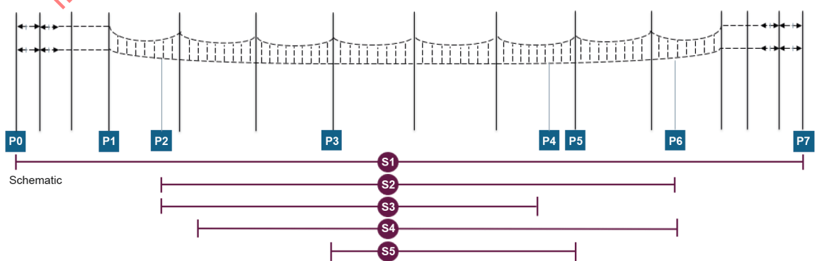
Figure E.2 – Defined points along the OCL (side view, idealized)
