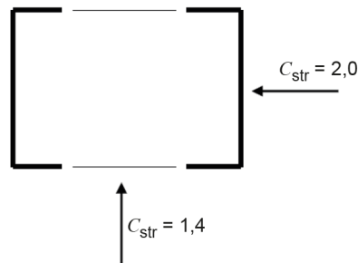
Figure 6 – Definition of drag factors for double channel structure pole
