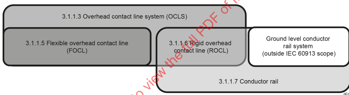
Figure 1 – Scope of contact line systems
