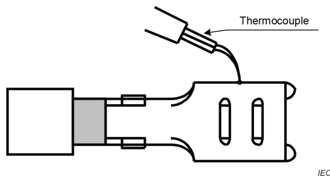
Figure I.1 – Example of position of the thermocouple for measurement of the temperature rise
