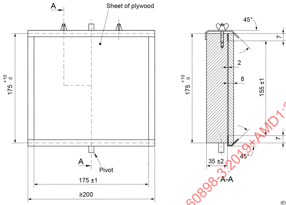
Figure 11 – Mounting support for mechanical impact test (see 9.13.2)
