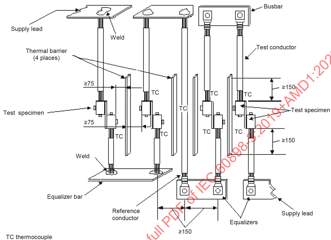
Figure J.1 – General arrangement for the test
