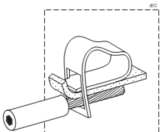
b) Screwless-type terminal with direct pressure
