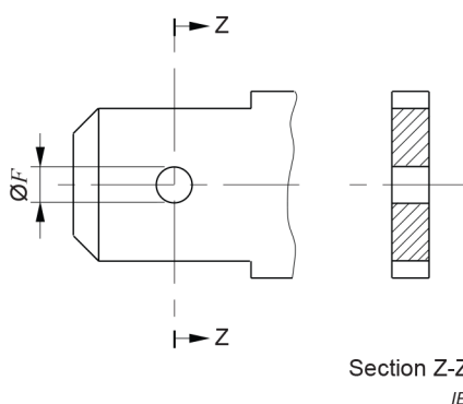
Figure I.4 – Dimensions of rectangular dimple detents (see Figure I.2)
