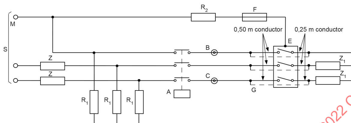
Figure 5 – Three-pole circuit-breaker with two protected poles and non-polarized protected M-pole
