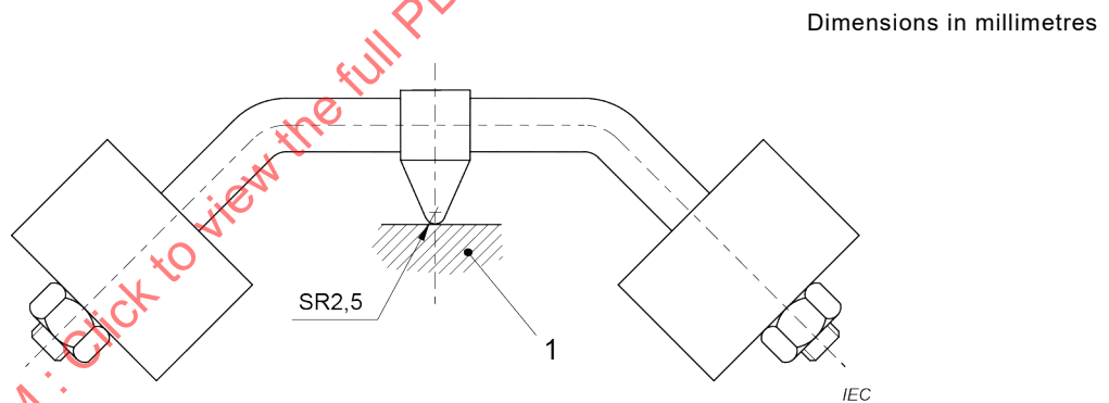
Figure 14 – Application of force for mechanical test on a rail-mounted circuit-breaker (see 9.13.2.4)
