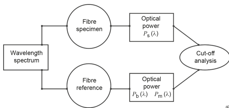
Figure 1 – Cut-off measurement system block diagram 2
