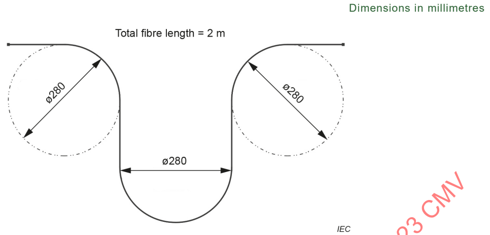
Figure C.2 – Alternative fibre cut-off deployment – Multi-bend
