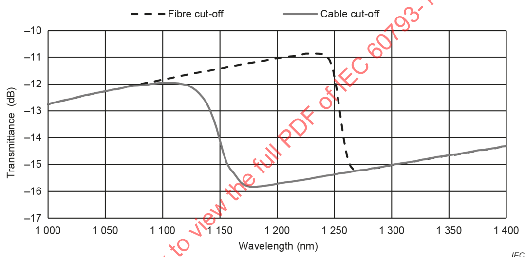
Figure 7 – Cable cut-off vs fibre cut-off for a specific fibre (multimode reference)
