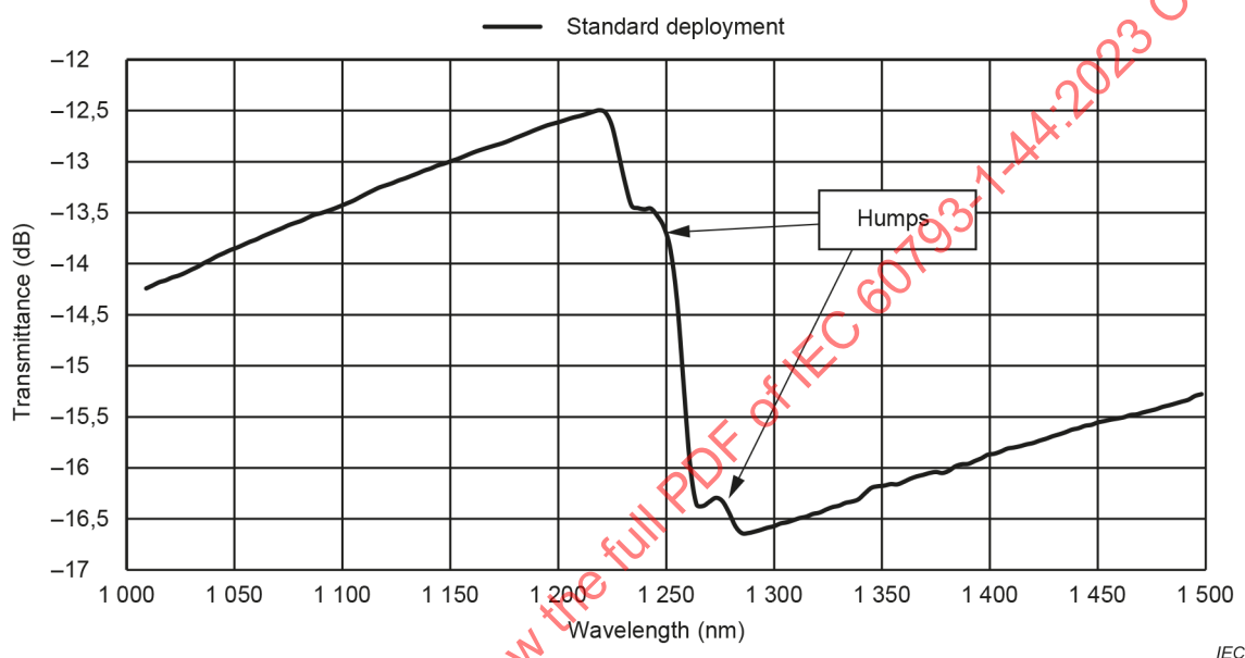
Figure D.4 – Fibre cut-off curve with artifacts (multimode reference)
