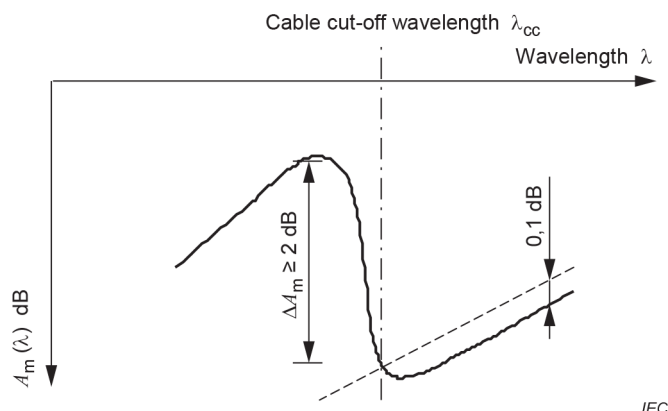
Figure 6 – Cut-off wavelength using the multimode-reference technique
