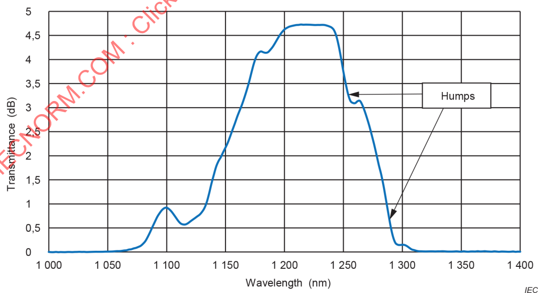
Figure D.5 – Fibre cut-off curve with artifacts (bend reference)
