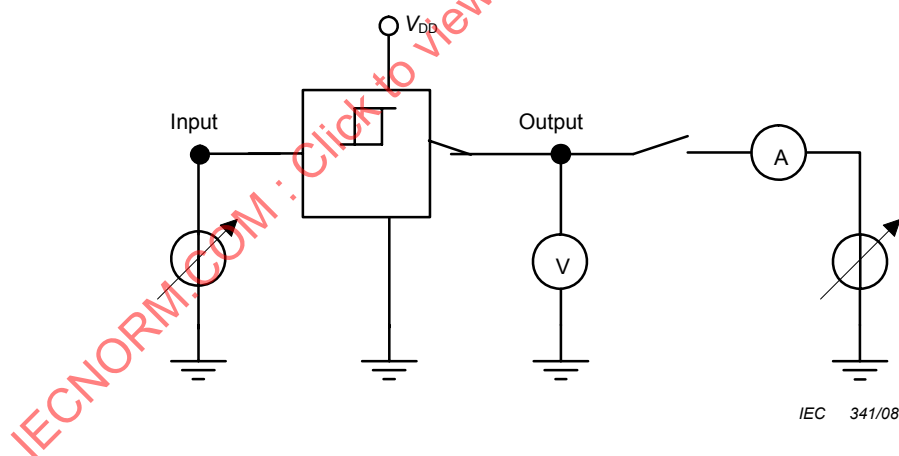
Figure A.1 – DC characteristic measurement circuit of Schmitt-trigger input
