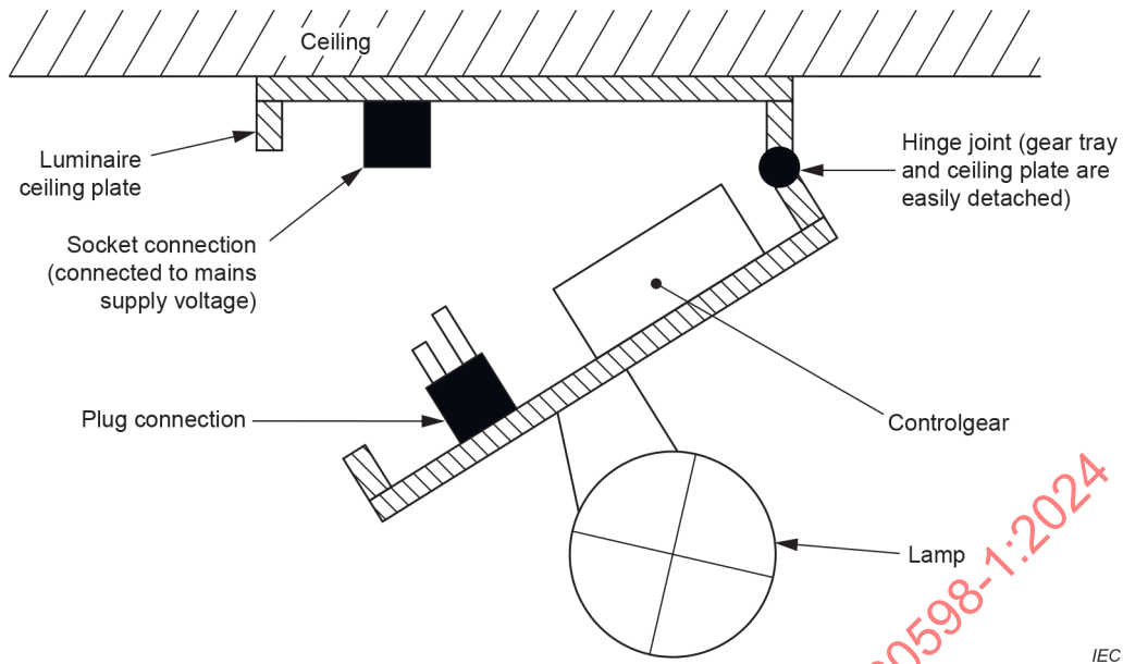
Figure 3 – Example of electro-mechanical contact system with plug or socket connection
