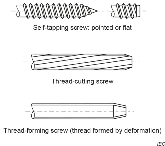
Figure 32 – Examples of self-tapping, thread-cutting and thread-forming screws
