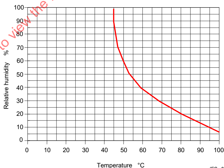
Figure 101 – Temperature/relative humidity characteristic during normal operation
