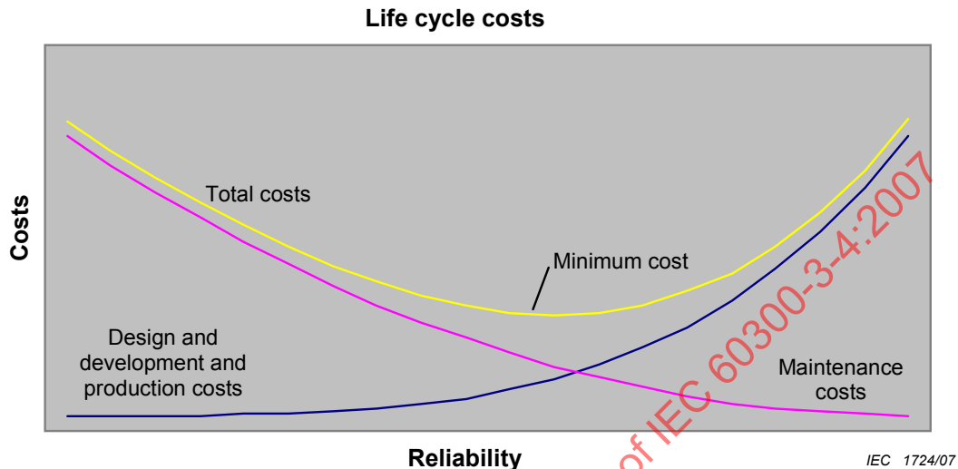
Figure 1 – Relationship between cost and reliability
