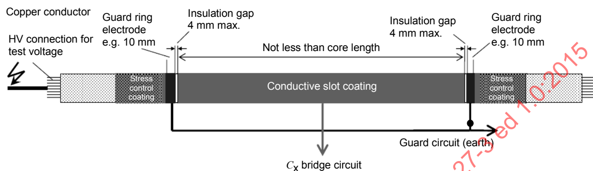
Figure 8 – Arrangement with guard rings electrodes on test objects with insulation gap (example of preferred insulation gap and guard electrode dimensions)
