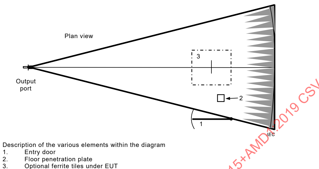
Figure I.2 – Typical GTEM plan sectional view showing floor layout
