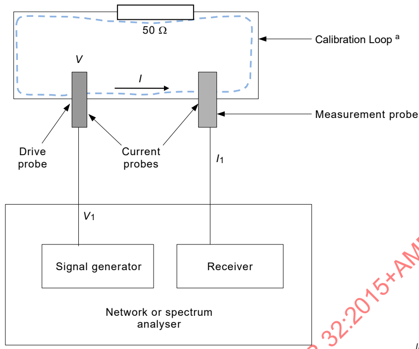
Figure C.6 – Calibration fixture
