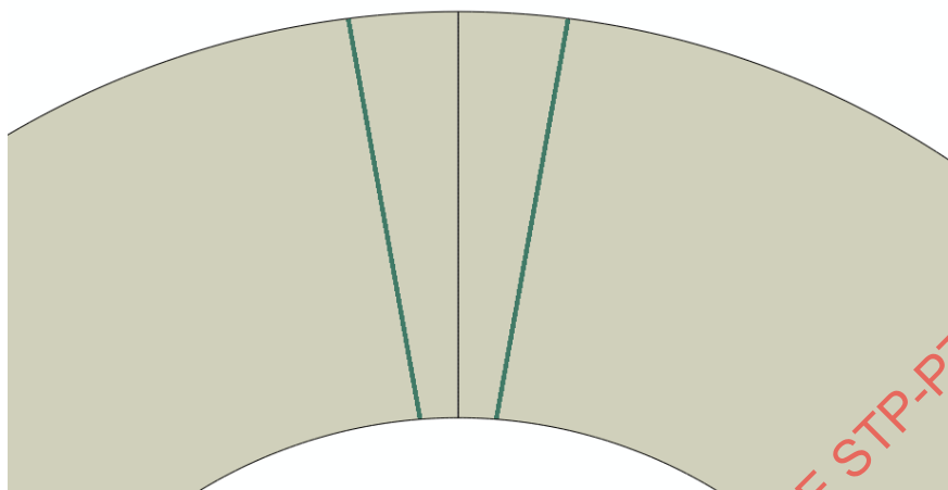
Figure 58: Seamweld HAZ Model Pipe OD = 762 mm, ID = 427 mm, Weak HAZ Width = 2 mm, Weld Semi-Angle = 10^{\circ}
