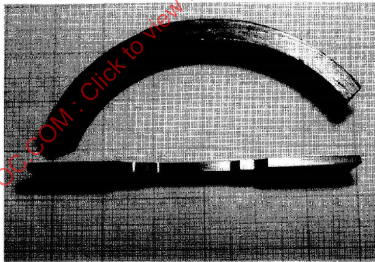
Figure 15. Flat specimen prepared from heater tube.
