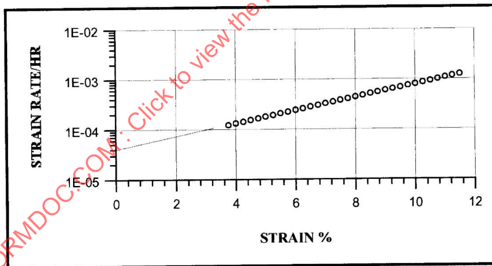
Figure 11. Illustration of the graphical determination of \dot{\epsilon}_0 from a partial creep curve.
