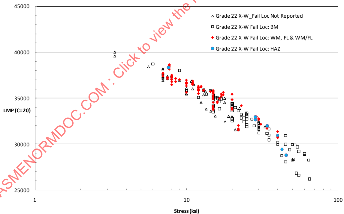
Figure 9: Grade 22 Cross-Weld (X-W) Specimen Stress Rupture Data from EPRI TR-110807 [10]
