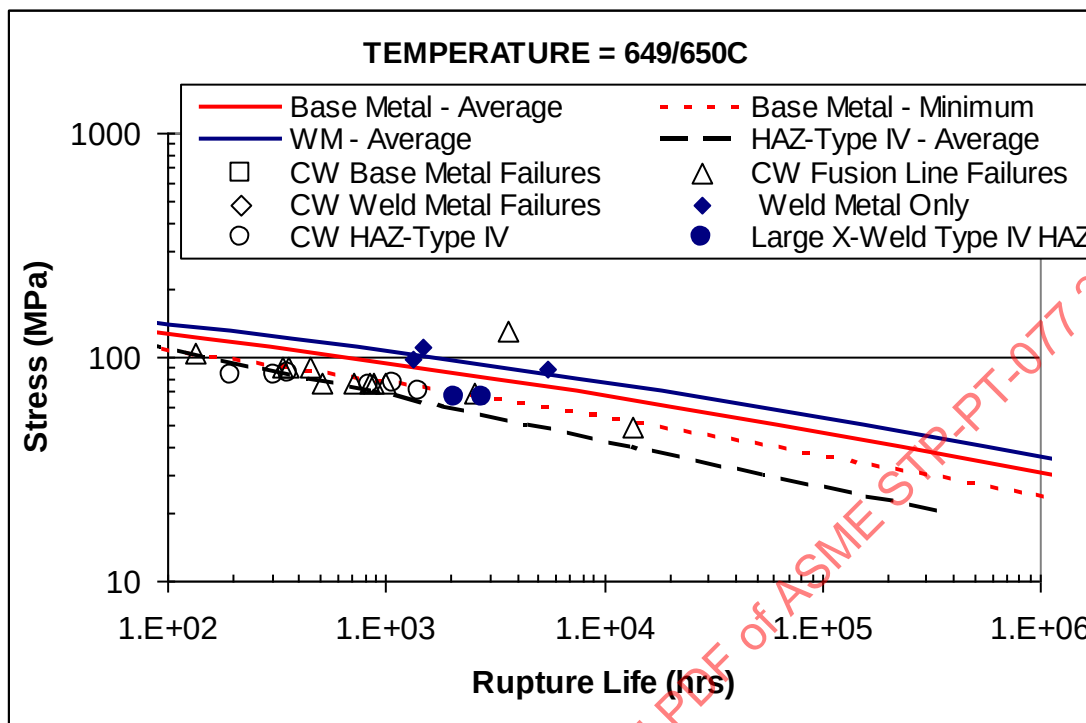
Figure 43: Comparison of Predictions in Figure 39 Plotted with Data at 649/650°C
