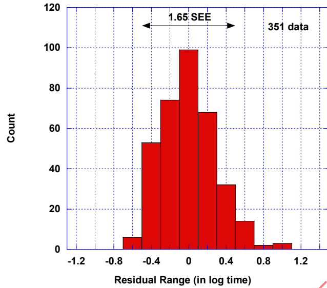
Figure 7 - Histogram of Residuals for Fit of LM Parameter for Alloy 800H
