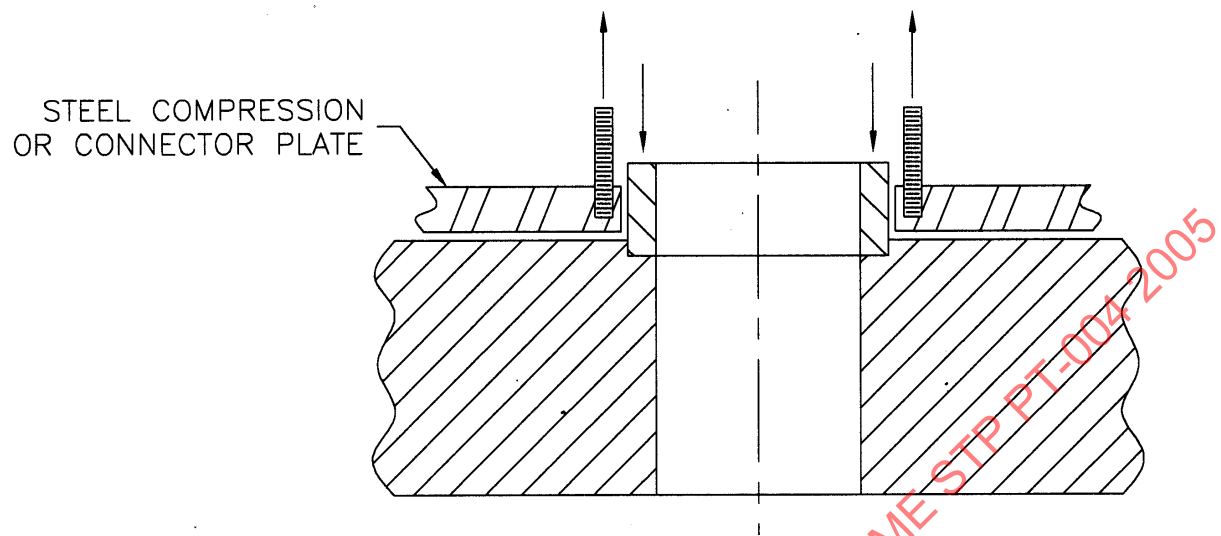
Figure 14 - Acceptable Nozzle Details in Graphite Vessels, Example D
