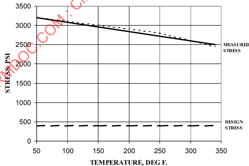
Figure 6 - Flexural Stress vs. Temperature
