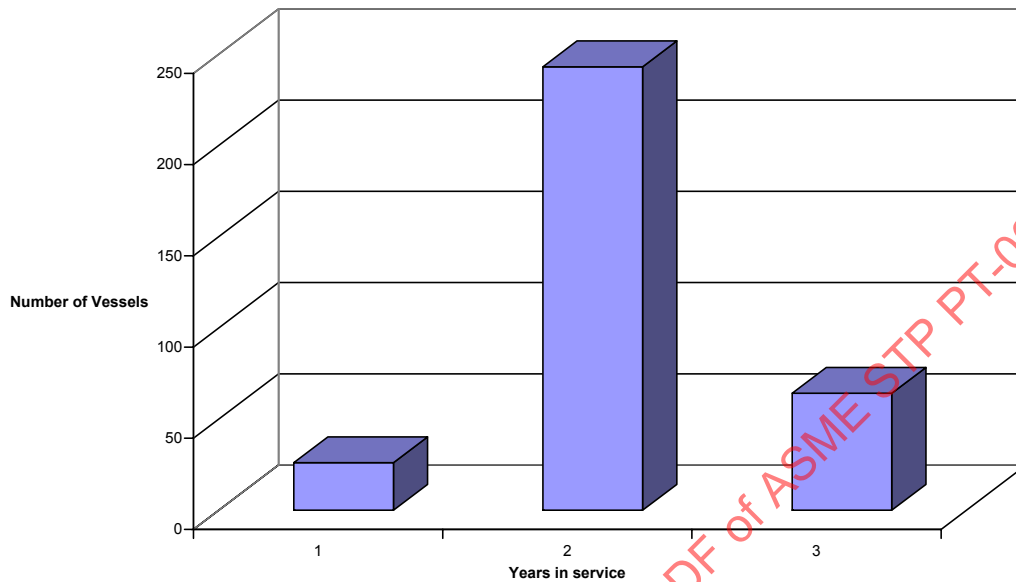
Figure 6 - Appendix 22 Storage Vessels (7,000 psig MAWP-10 in. OD)
