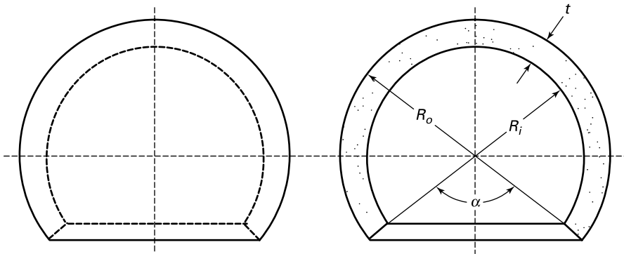
(a) Hyperhemispherical Window
