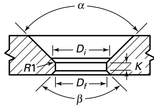
Figure 2-2.9.1-1 Seat Cavity Requirements — Conical Frustum Window, Spherical Sector Window With Conical Edge, and Flat Disk Window
