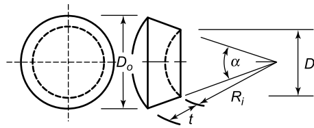
(a) Spherical Sector Window With Conical Edge
