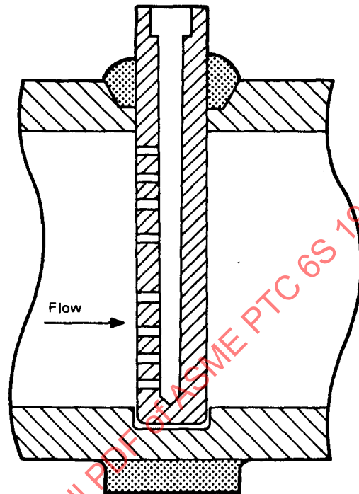
FIG. 4.5 MOISTURE-SAMPLING TUBE
