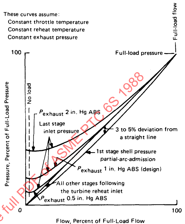
FIG. 6.5 PRESSURE-FLOW RELATIONSHIP
