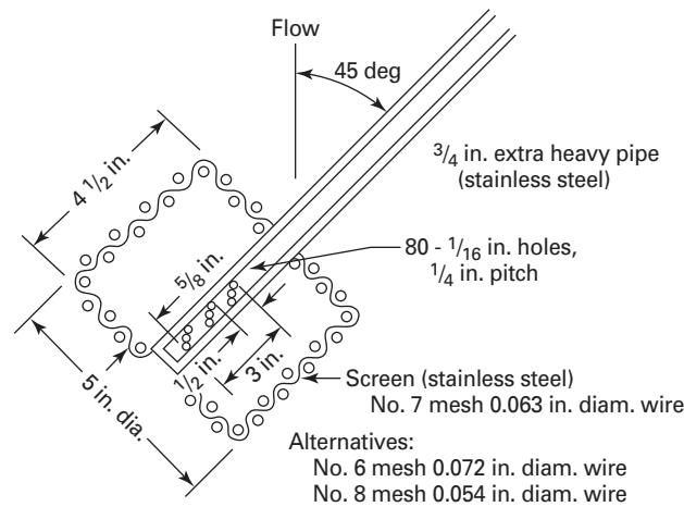
Fig. 4-2.7.3-1 Basket Tip
