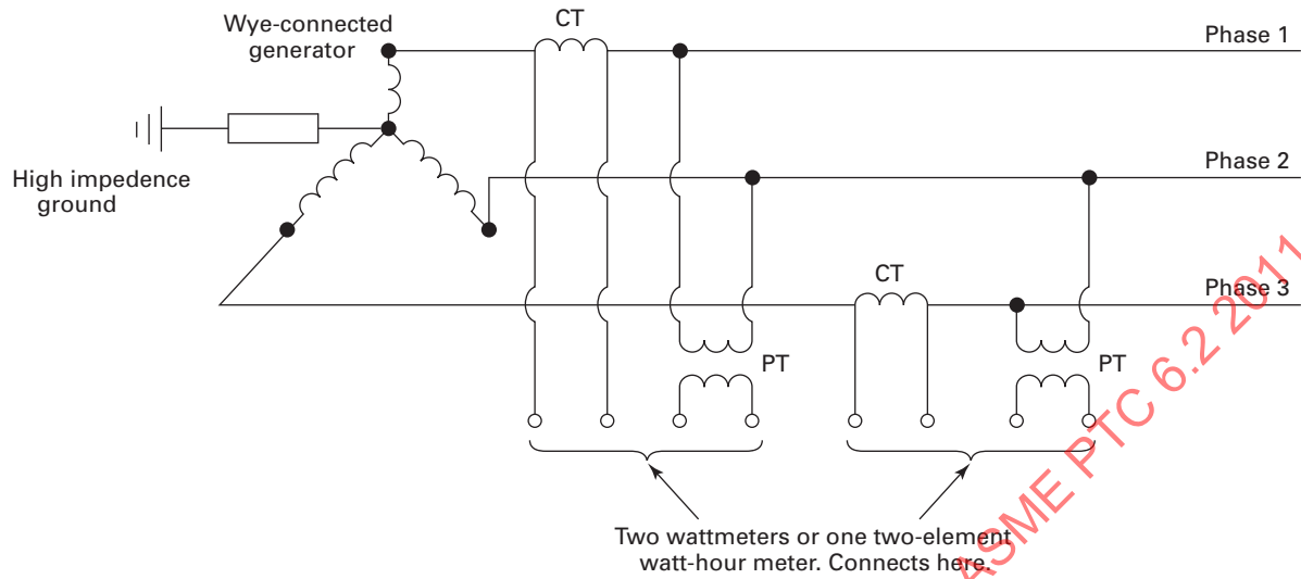
Fig. 4-5.2.1-2 Two-Meter System for Use on Three-Wire Wye-Connected Power Systems
