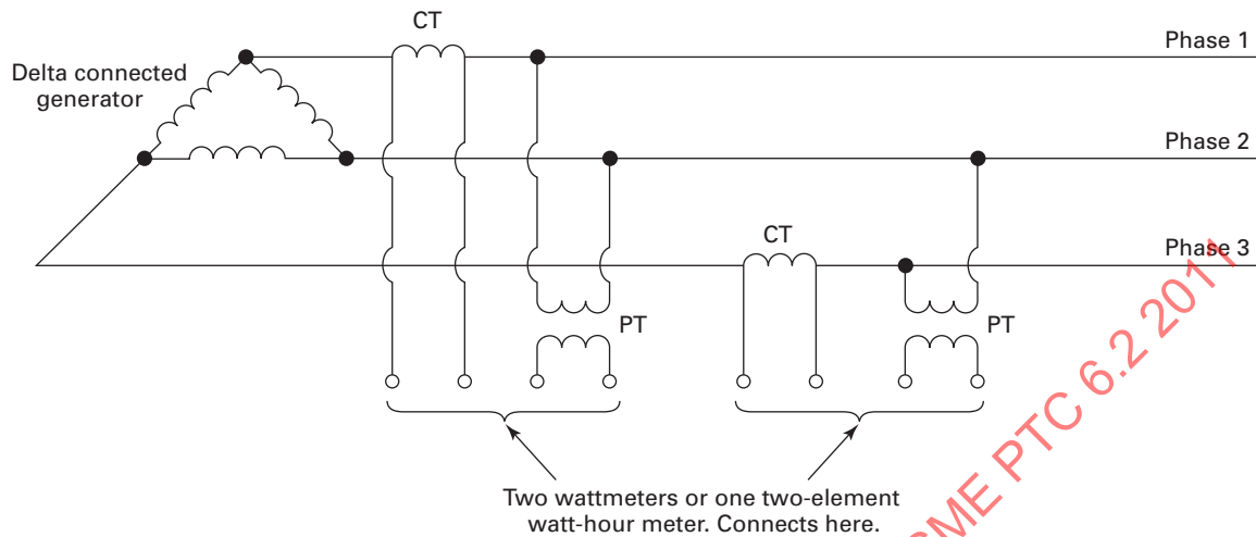
Fig. 4-5.2.1-1 Two-Meter System for Use on Three-Wire Delta-Connected Power Systems
