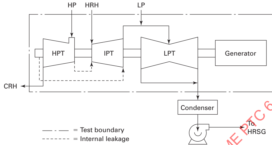
Fig. 3-1.2-1 Three-Pressure Reheat Steam Turbine Heat Balance
