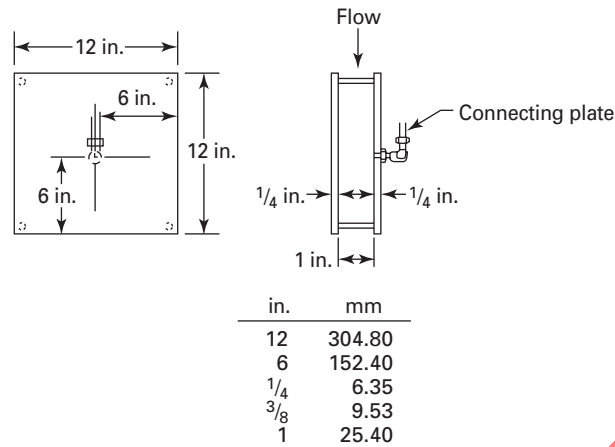
Fig. 4-2.7.3-2 Guide Plate
