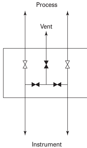
Fig. 4-2.6.2-1 Five-Way Manifold
