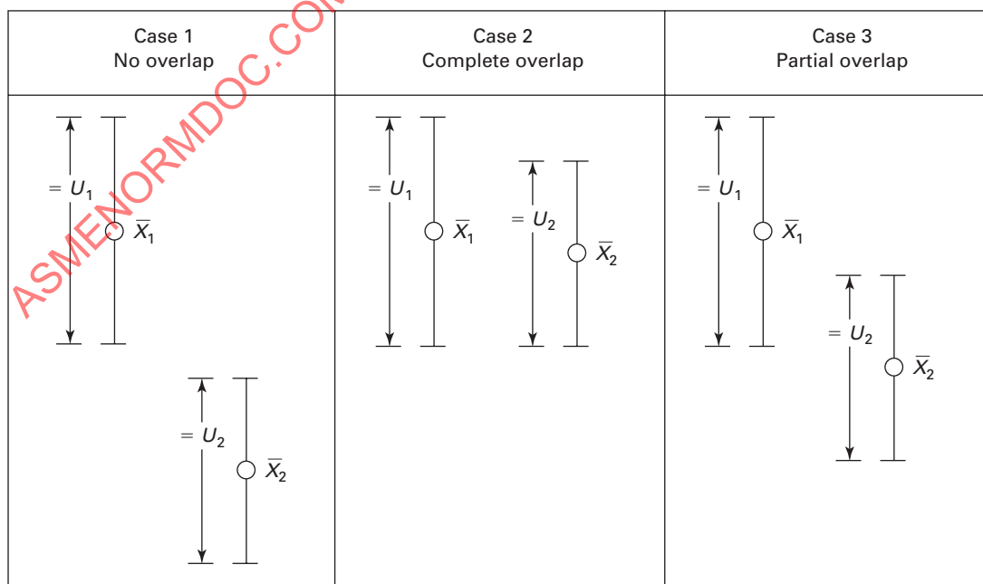
Fig. 3-5.5.3 Uncertainty Intervals
