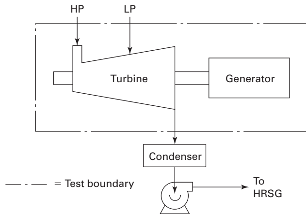
Fig. 3-1.2-2 Two-Pressure Nonreheat Steam Turbine Heat Balance
