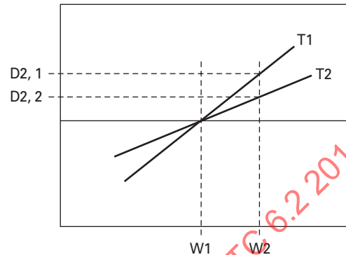
Fig. 5-3.2.1 Illustration of a Correction Curve With Independent and Interacting Variables
