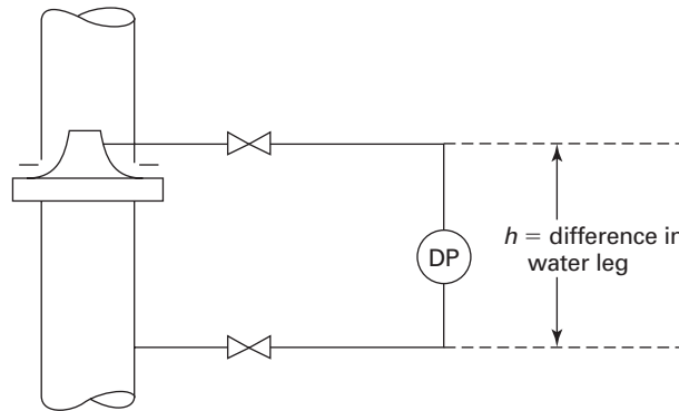
Fig. 4-2.6.2-2 Water Leg Correction for Flow Measurement
