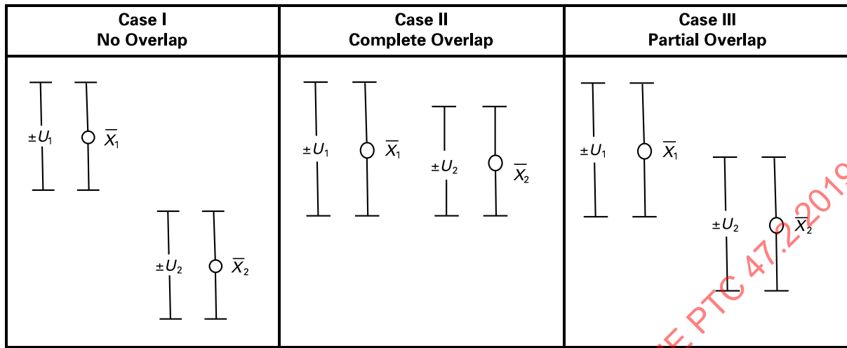
Figure 3-5.9-1 Uncertainty Intervals
