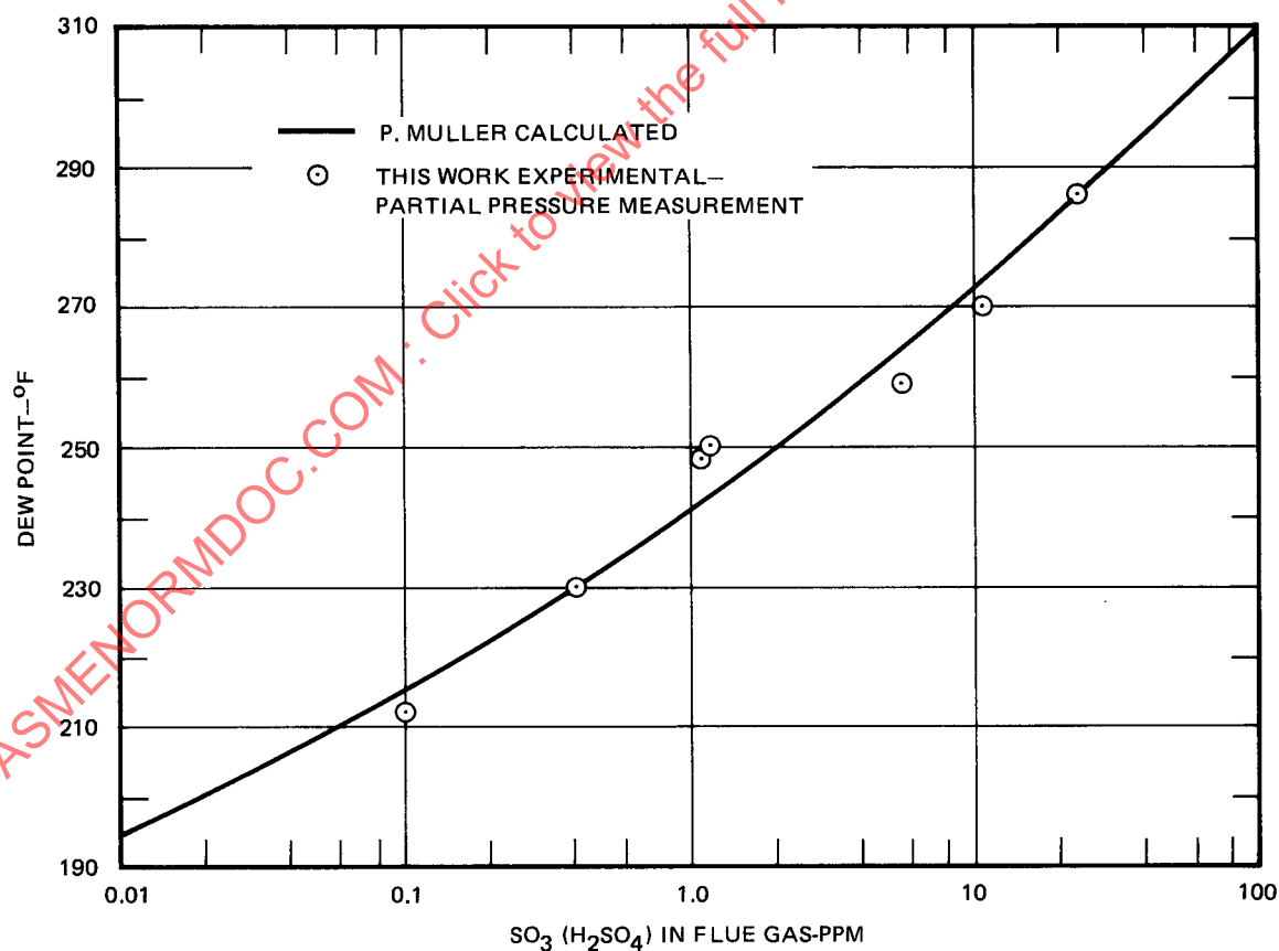
FIG. F-2 DEW POINT AS A FUNCTION OF H 2 SO 4 CONCENTRATION
