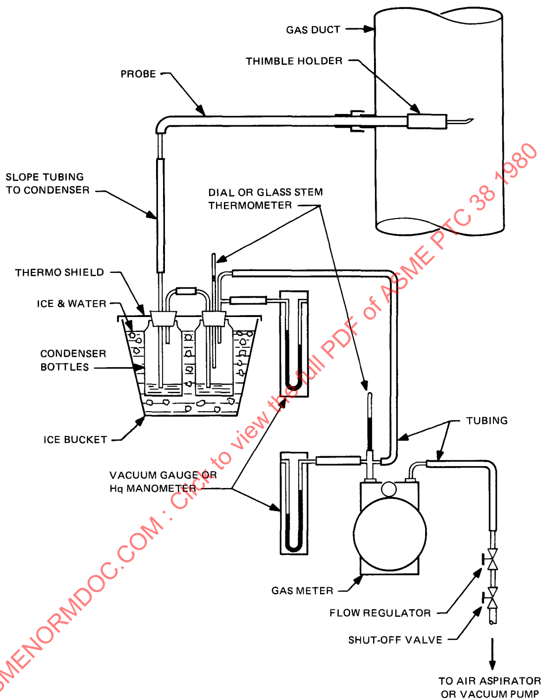
FIG. 5-2 MOISTURE DETERMINATION — CONDENSATE METHOD
