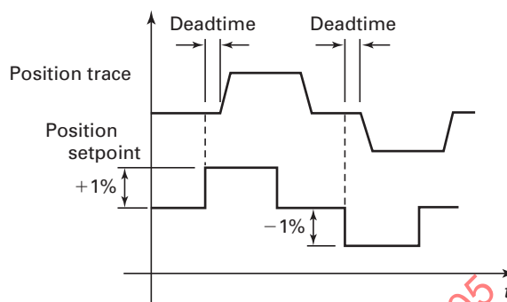
Fig. 4-4 Position Deadtime
