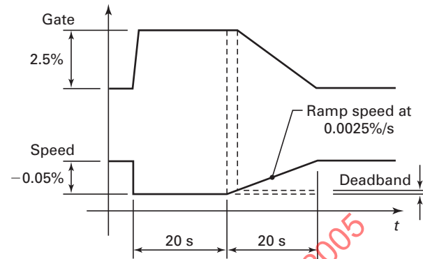
Fig. 4-2 Speed Deadband
