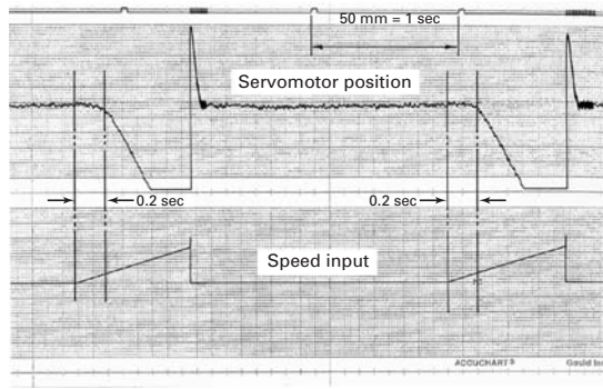
Fig. 5-2 Speed Deadtime
