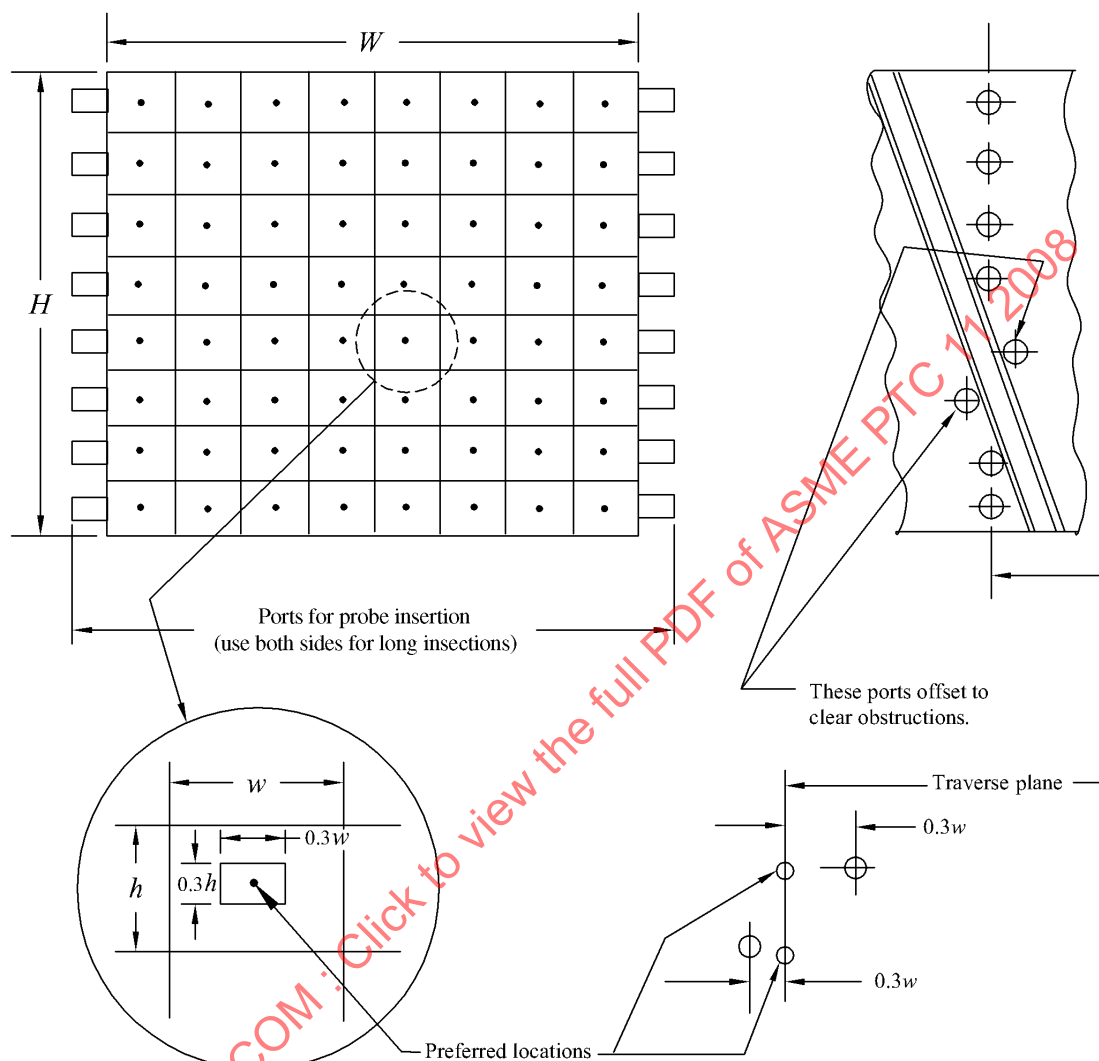
Fig. 4-2.4-1 Sampling Point Details (Rectangular Duct)
