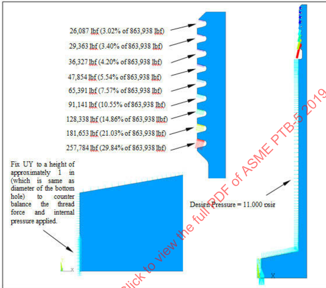
Figure 27 – E-KD-2.3.1-4 – Load and Boundary Conditions for the FE Model
