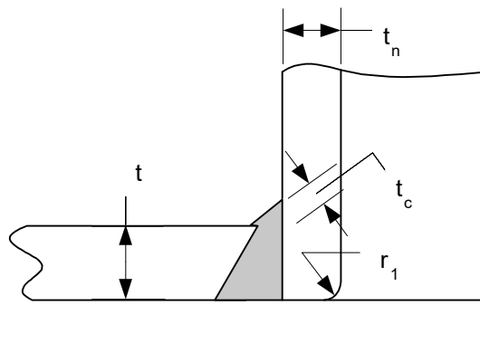
Figure E4.2.2 – Weld Details
