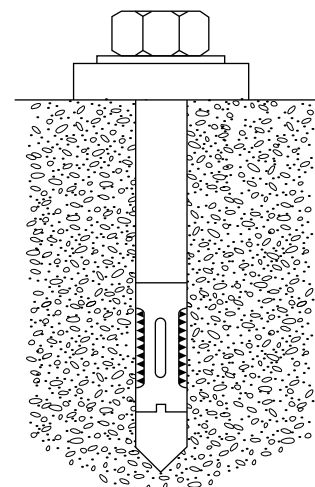
Figure 308-4.3.2-1 Sleeve Anchor
