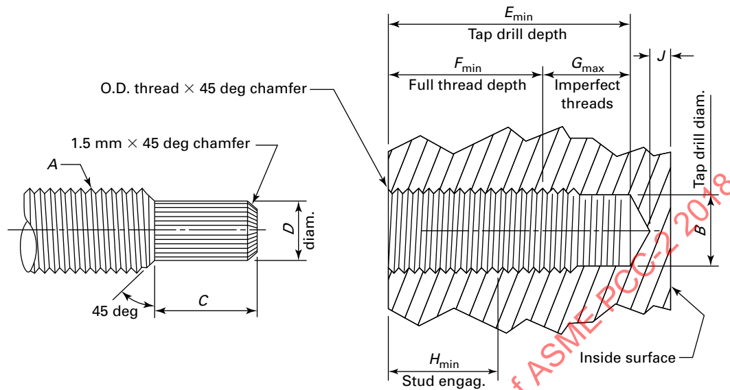
Figure 303-I-3 Metric Thread Series (SI Units)
