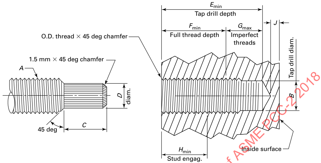
Figure 303-I-2 Inch Thread Series (SI Units)
