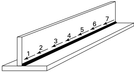
Figure 208-4.2-1 Typical Back Stepping Weld Sequence
