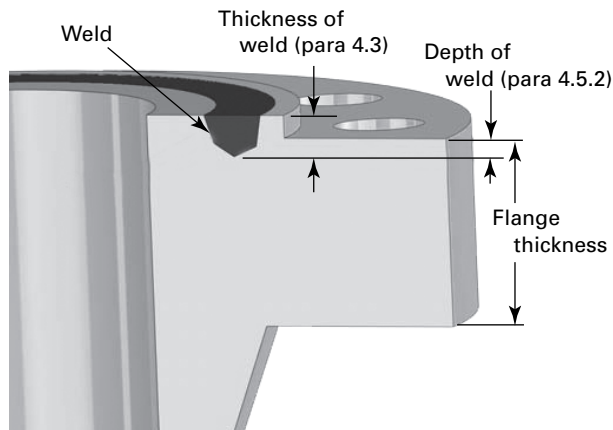
Figure 305-4.5.2-1 Flange Dimensions
