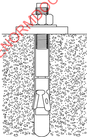
Figure 308-4.3.1-1 Wedge Anchor
