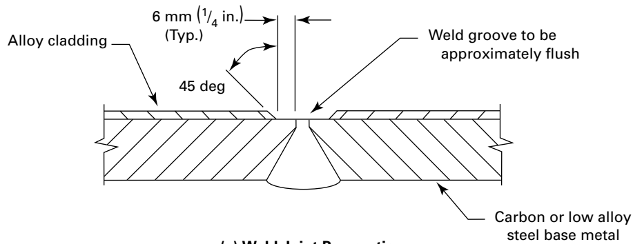
Figure 211-4.4.1-1 Weld Seam With Back Cladding
