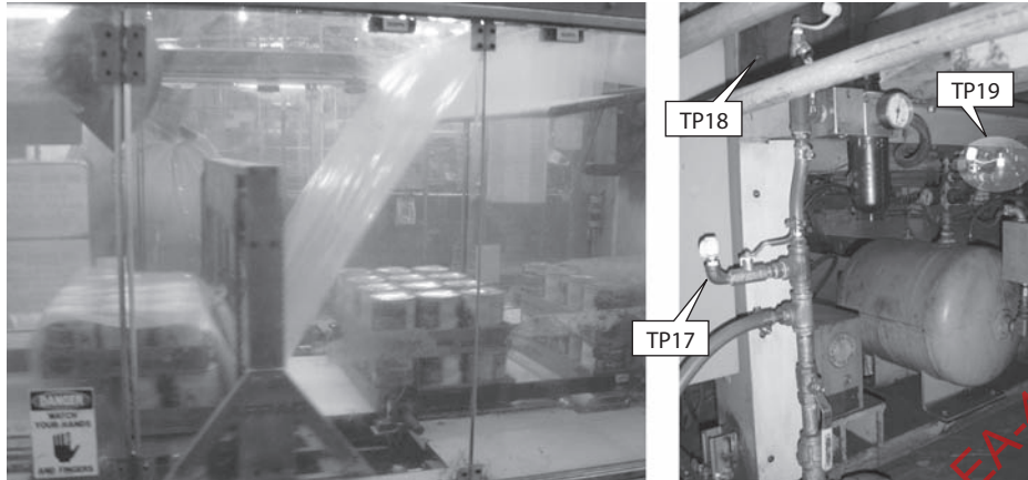
Fig. 12 Wrapper Machine and Test Pressure Locations TP17, TP18, and TP19
