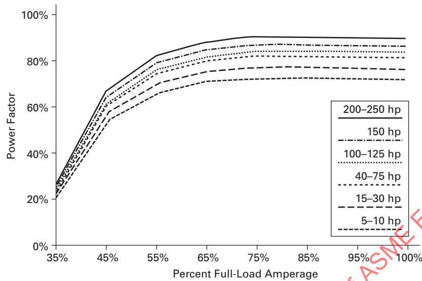
Fig. 2 Motor Power Factor as a Function of Percent Full-Load Amperage
