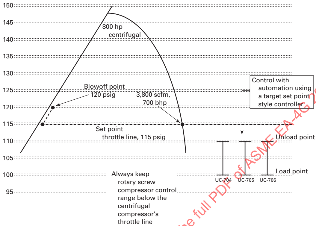
Fig. 6 Example Pressure Profile 2
