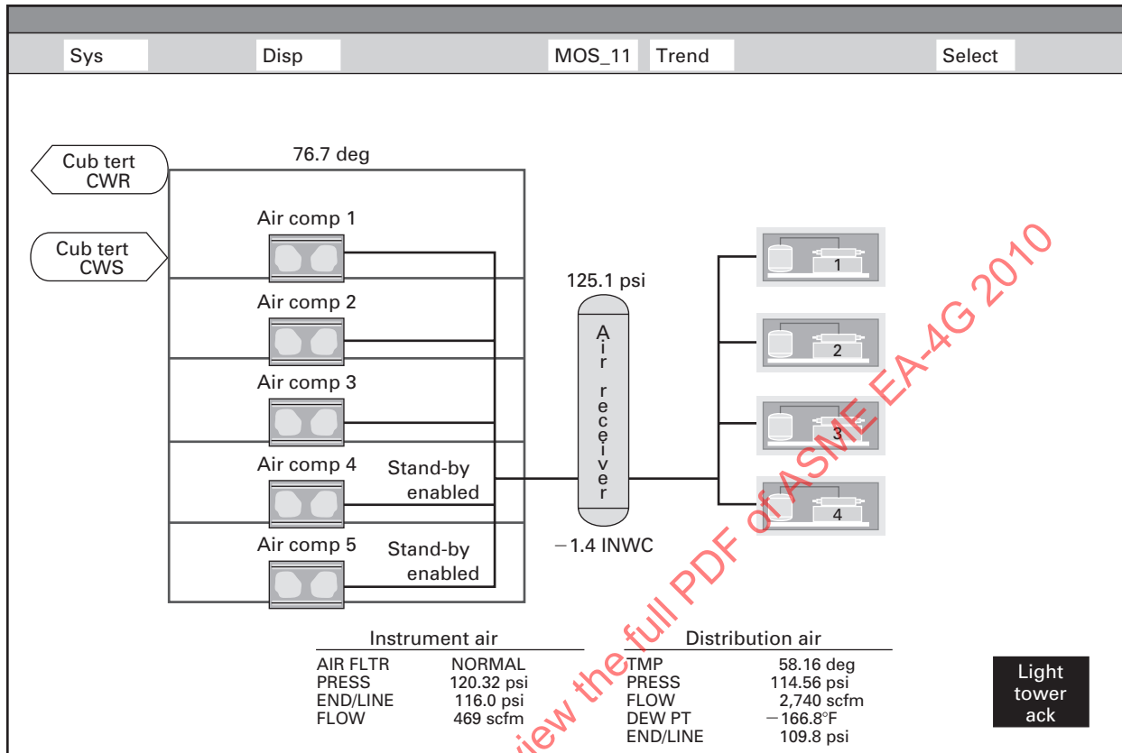
Fig. 4 Example Installed Data System
