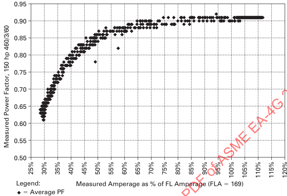
Fig. 3 Measured Power Factor Versus Percent Full-Load Amperage
