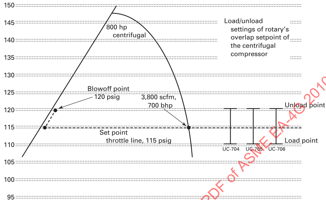
Fig. 5 Example Pressure Profile 1
