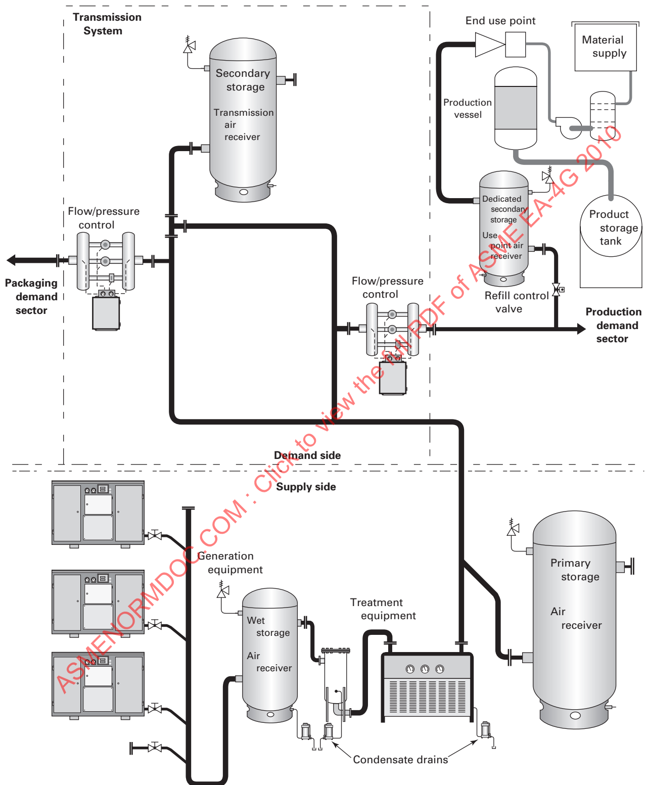
Fig. 1 Example Compressed Air System
