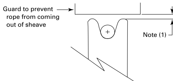
Fig. 4-2.7-1 Sheave Gap
