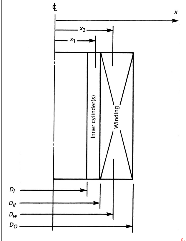
Figure KD-911 Nomenclature for Wire-Wound Cylinders
