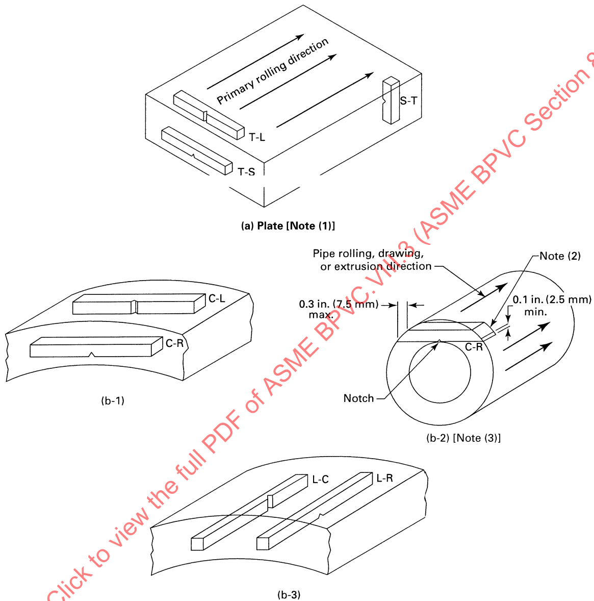
(b) Charpy V-Notch Specimens From Pipe [Note (4)]
