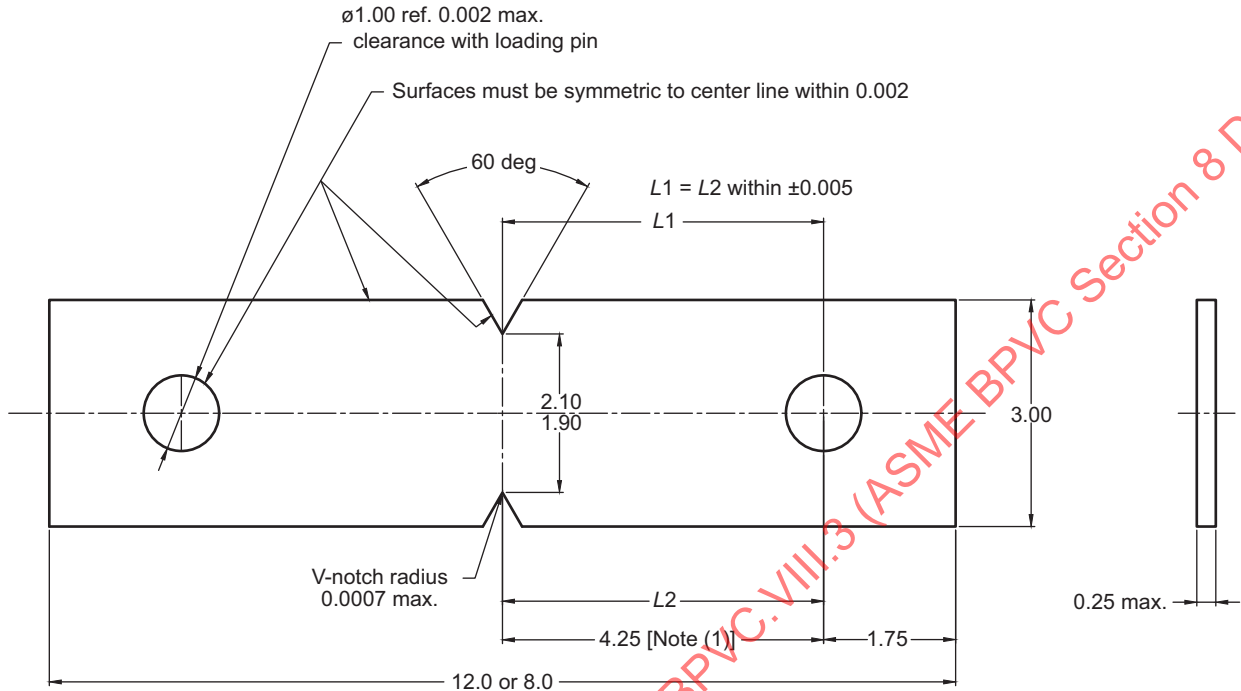
Figure KM-270.1 Machine Sharp Edge-Notch Specimen
