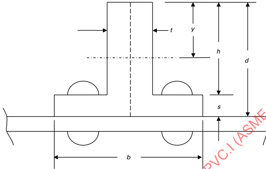
Figure PL-36.9-1 Tee Iron
