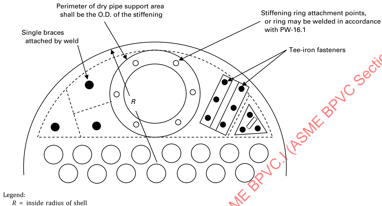
Figure PL-36.2.1-1 Support Perimeters
