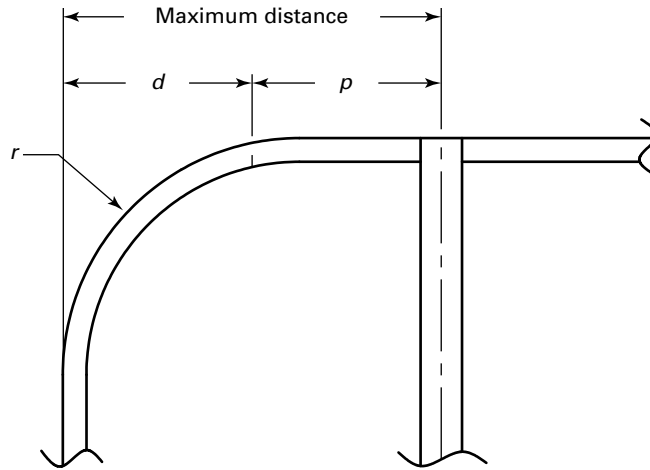
Figure PFT-27.2-1 Maximum Spacing as Defined in PFT-27.2
