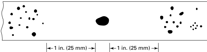
(b) Isolated Indication [Note (2)]
