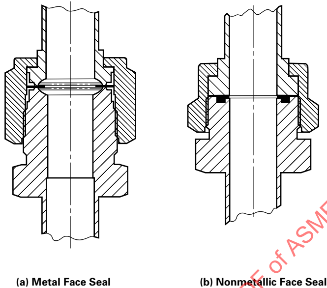
Figure U335.7.1-1 Face Seal Joints
