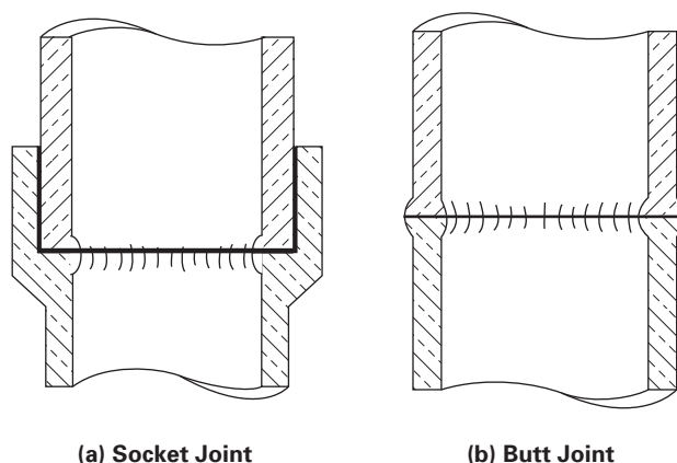
Fig. N-127.7.2(B) Heat Fusion Joints
