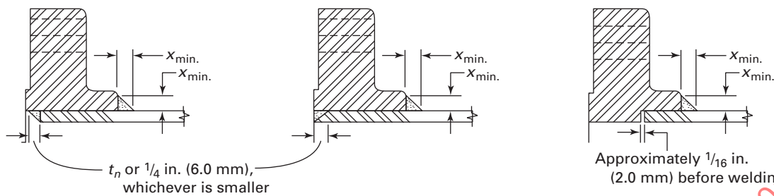
(a) Front and Back Weld [See Notes (1) and (2)]
