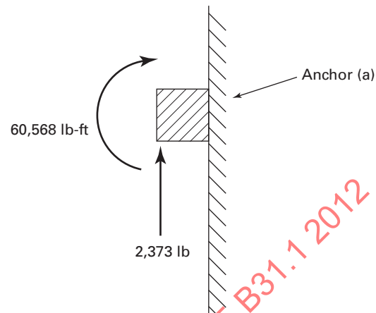
Fig. II-7-3 Sample Problem Figure 3
