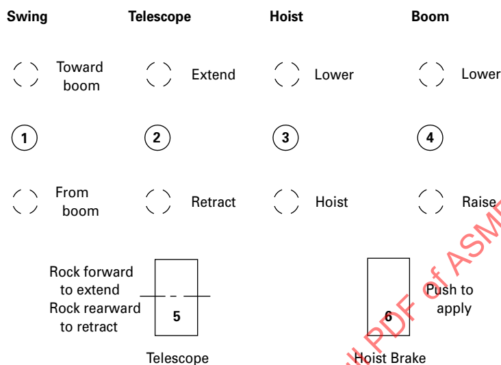
Fig. 5-1.6.1-1 Telescopic Boom Crane Control Diagram (Suggested Mobile Telescopic Boom Crane Basic Operating Control Arrangement for New Cranes)
