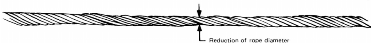
Fig. 5-2.4.2-1 Core Failure in 19 × 7 Rotation-Resistant Rope
