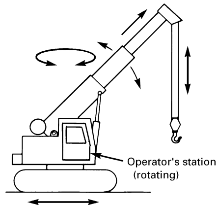
Fig. 5-0.2.1-4 Crawler Crane — Telescoping Boom
