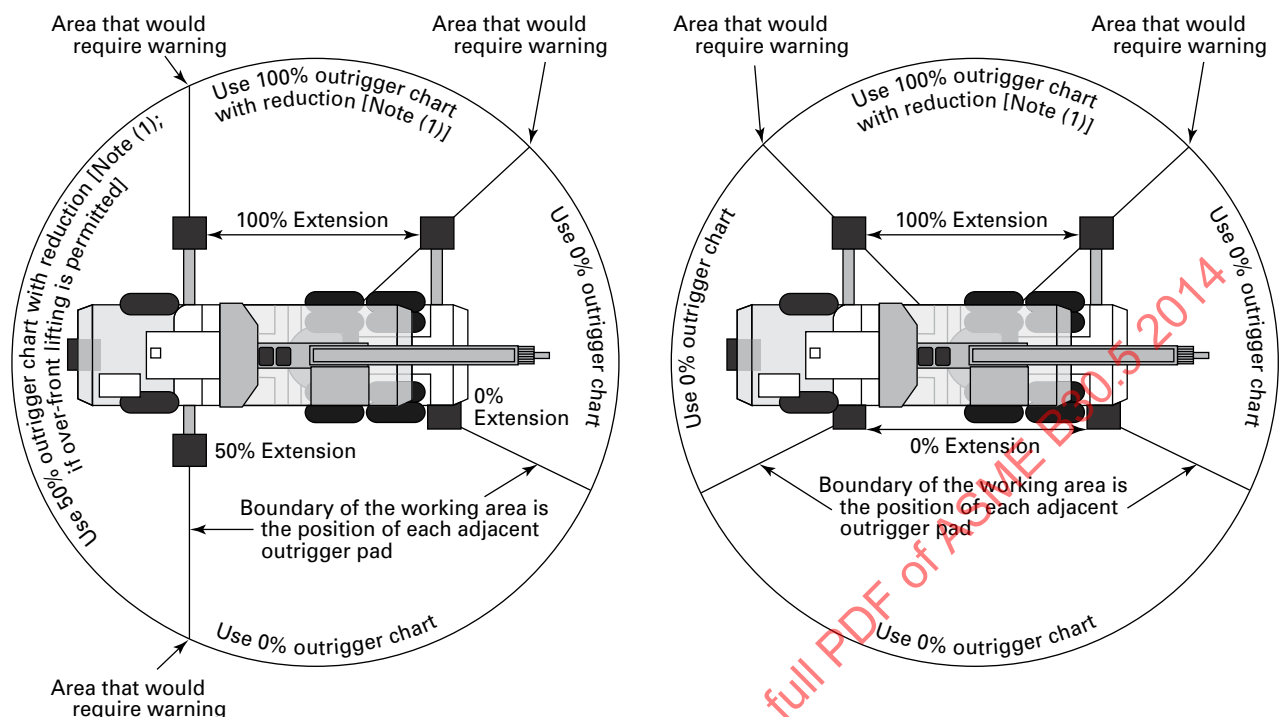
Fig. 5-3.2.1.5-1 Examples of Typical Unequal Outrigger Extension Positions
