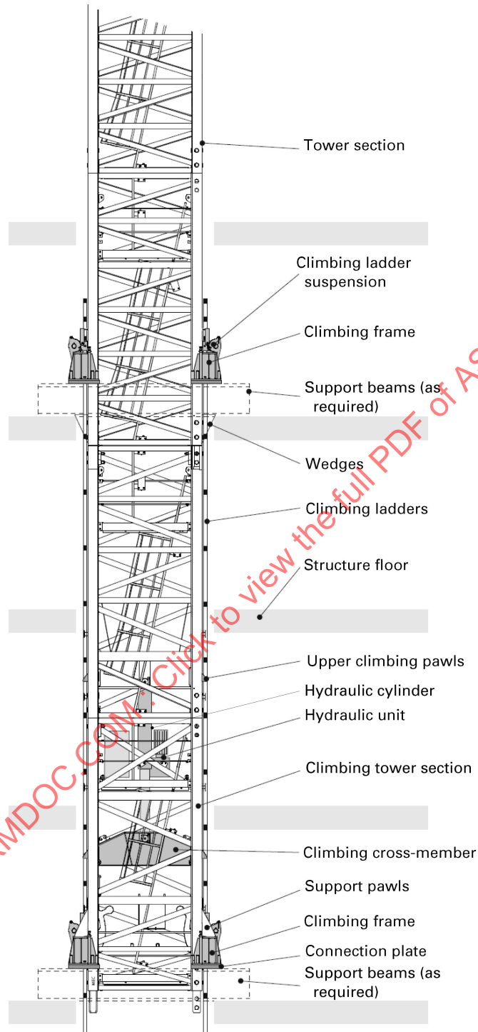
Figure 3-0.2.1.3-2 Internal Climbing Crane
