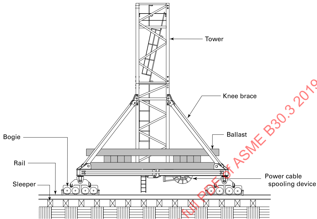
Figure 3-0.2.1.4-1 Travel Base for Freestanding Crane
