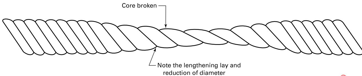
Figure 3-2.4.2-1 Core Failure in Rotation-Resistant Rope
