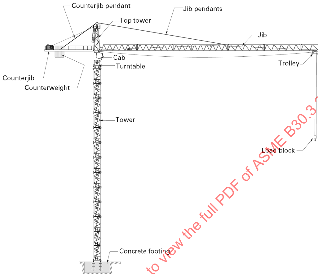
Figure 3-0.2.1.2-1 Hammerhead Tower Crane — Fixed-Base, Freestanding Crane
