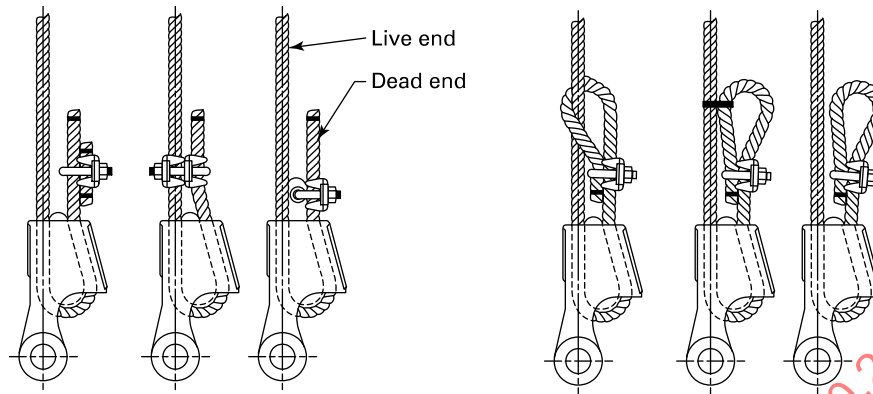
Figure 29-1.14-1 Wedge Sockets
