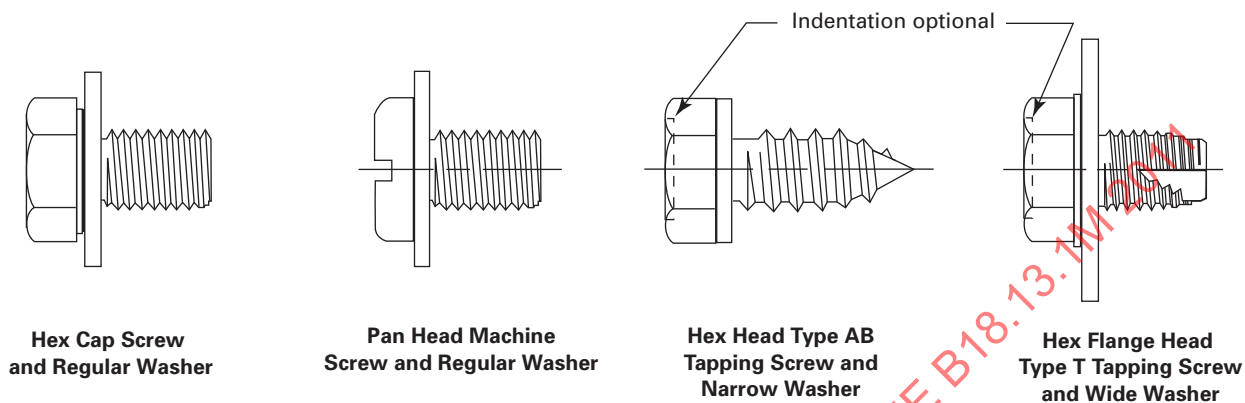
Representative Examples of Plain Washer SEMS
