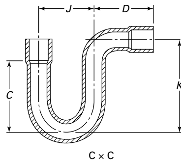
Suction Line P-Trap
