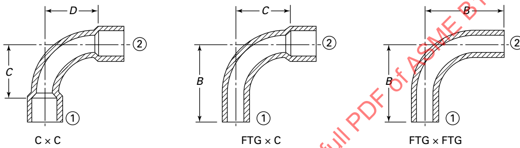
90-deg Elbows — Long Radius
