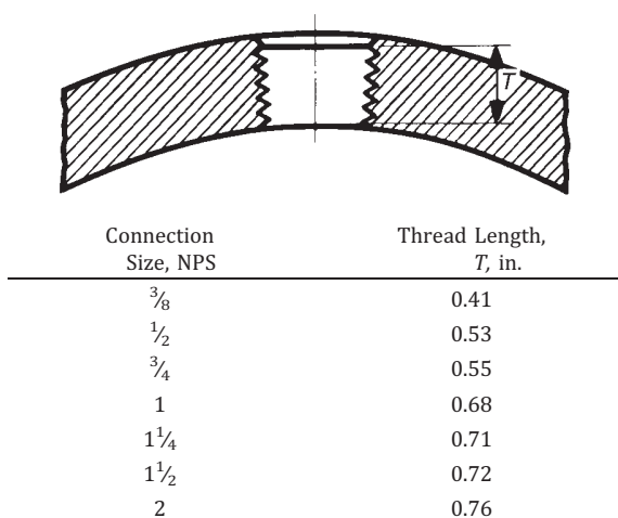
Figure II-11 Thread Length for Connection Tapping
