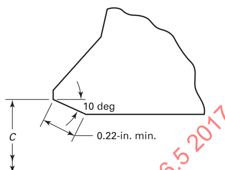
Figure II-10 Inside Contour for Use With Taper Backing Ring
