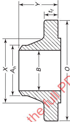
Welding Neck
