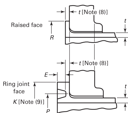
Lap Joint Stub End Facings and Thickness Lapped Joints
