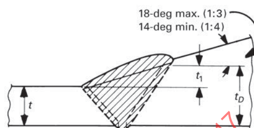
Figure 1 Bevel for Outside Thickness
