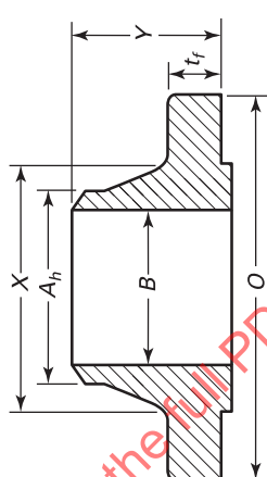
Welding Neck
