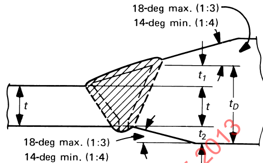
Fig. 3 Bevel for Combined Thickness
