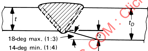
Fig. 2 Bevel for Inside Thickness
