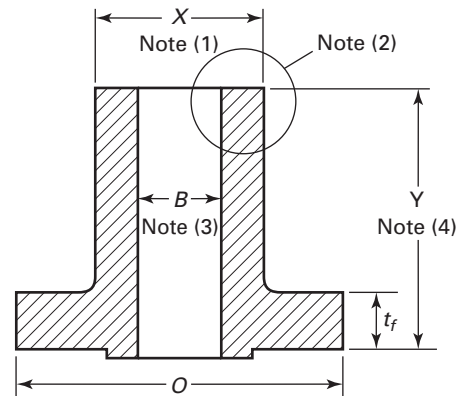
Fig. 4 Straight Hub Welding Flanges
