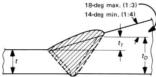
Fig. 1 Bevel for Outside Thickness
