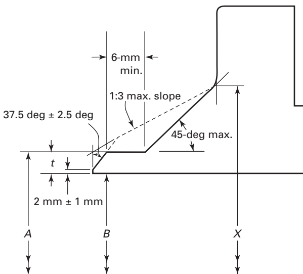
Fig. 7 Bevel for Wall Thicknesses t From 5 mm to 22 mm Inclusive
