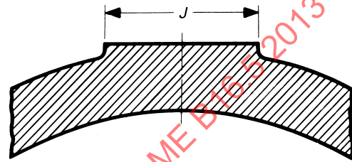
Fig. 13 Bosses for Connections
