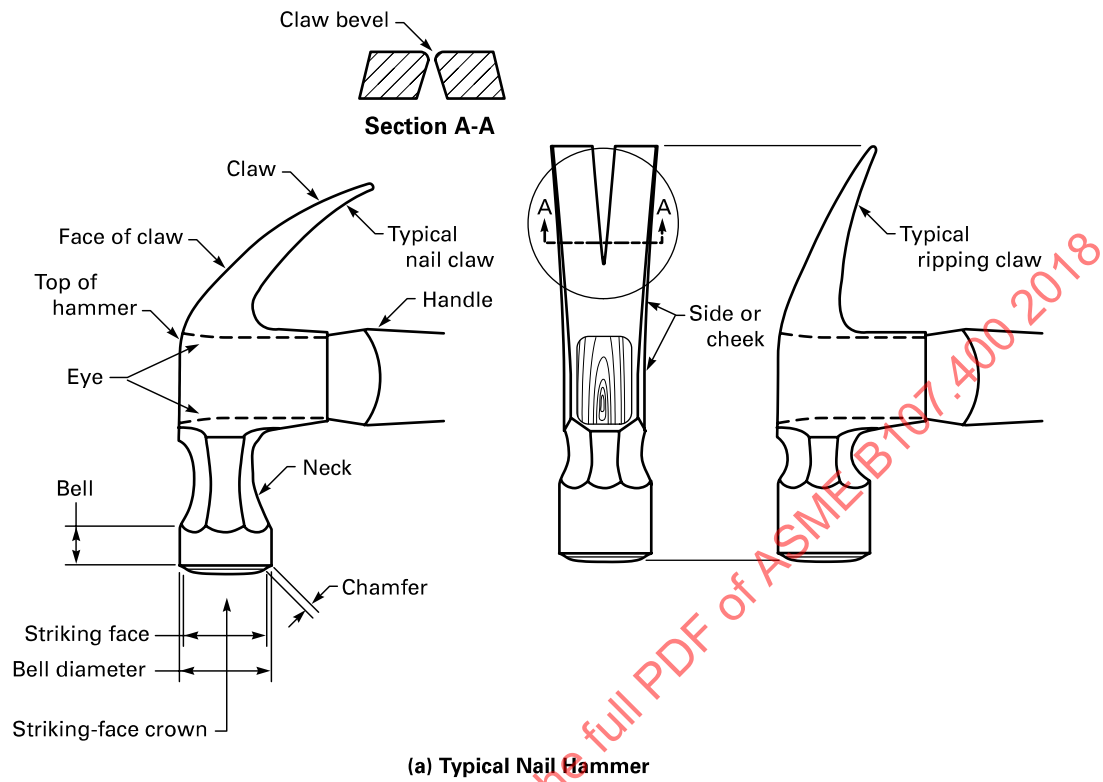
Figure 5.1-1 Category 41 Nail Hammer Nomenclature
