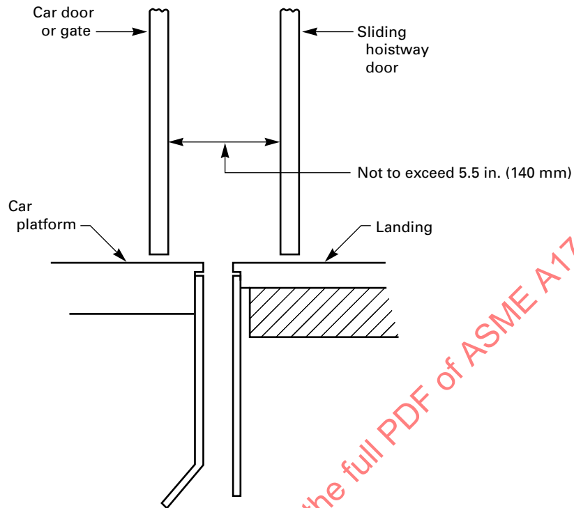
Figure A-2 Distance Between Sliding Hoistway Doors and Car Doors and Gates
