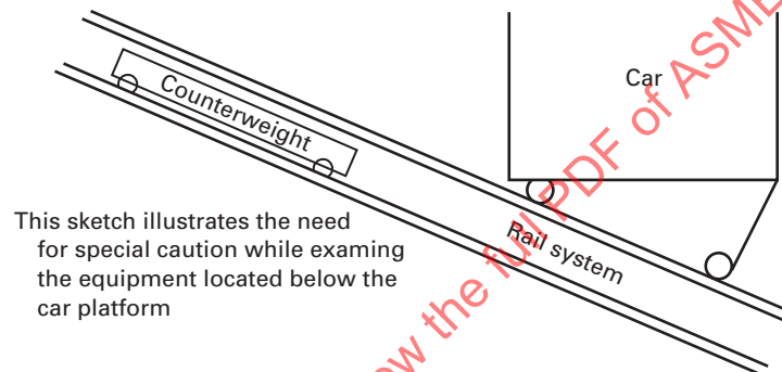
Fig. I-3.4 Uphill Clearance
