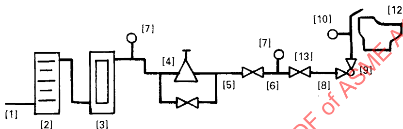
Water supply system shown ready for water closet test
