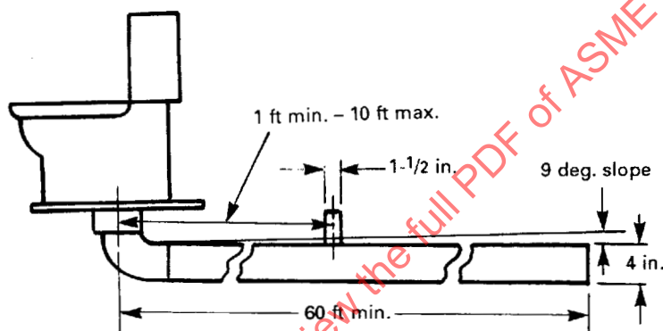
FIG. A-7 DRAINLINE TRANSPORT CHARACTERIZATION TEST ASSEMBLY
