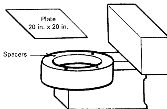
FIG. A-6 TEST PLATE (Applicable to para. 7.1.9.1)
