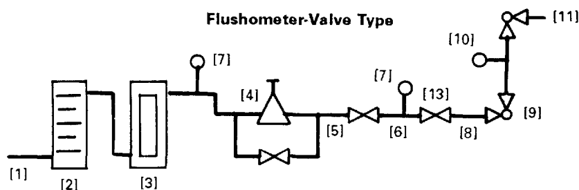
Water supply system shown ready for standardization
